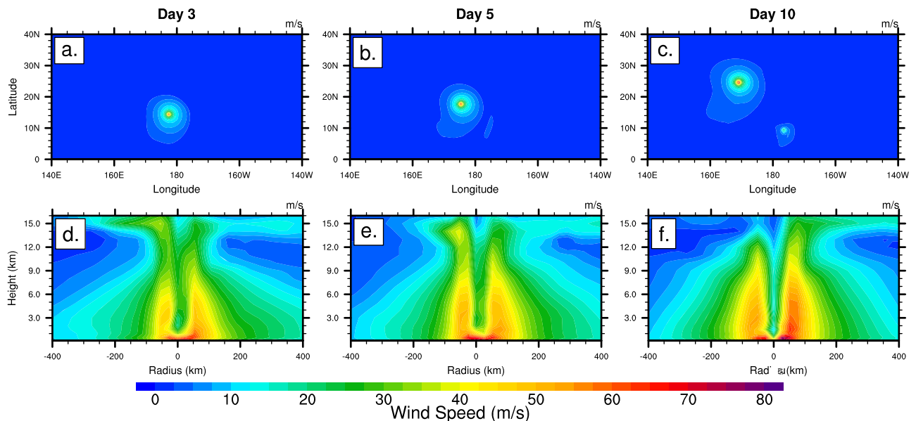
Figure 4. Snapshots of the tropical cyclone at (left) day 3, (middle) day 5 and (right) day 10 with CAM 5 FV at the resolution 0.25° L30 for simple-physics. (a–c) Horizontal cross section of the wind speed at a height of 100 m. (d–f) Longitude-height cross section of the wind speed through the center latitude of the vortex as a function of the radius from the vortex center.
